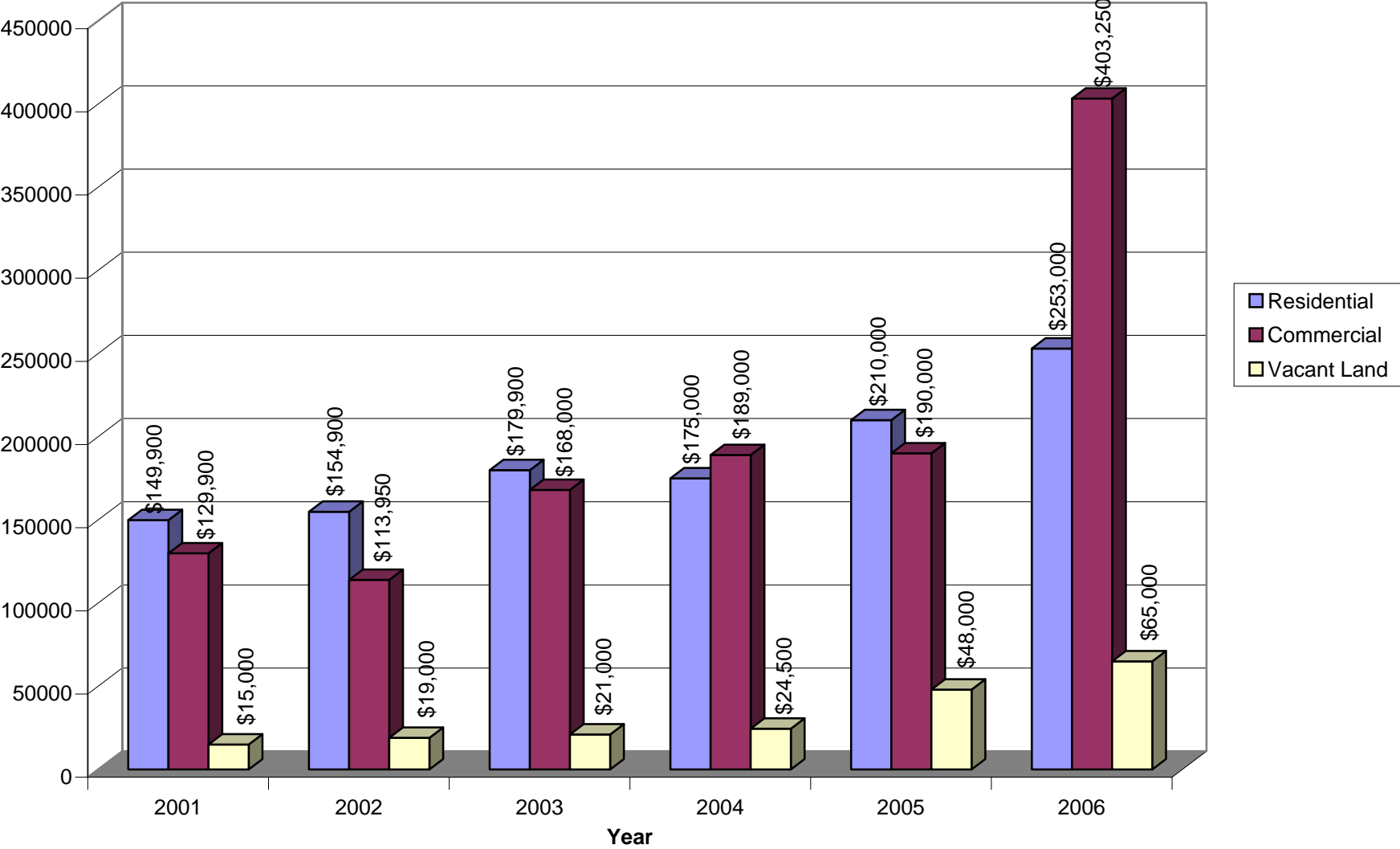
Median Price 2001-2006
